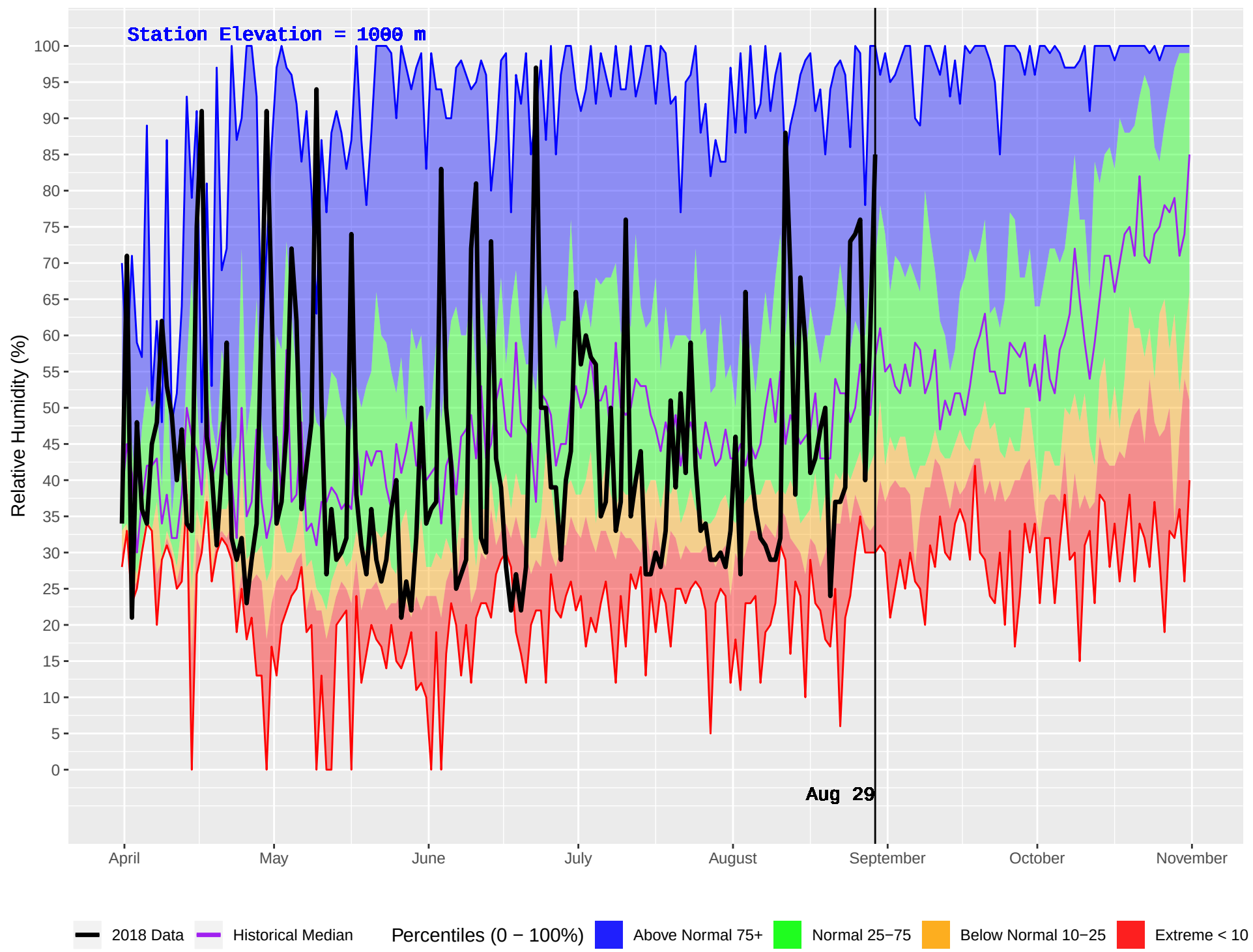
SUCCOUR CREEK (374) : Historical (1986–2016) and Current (2018) Daily Relative Humidity
