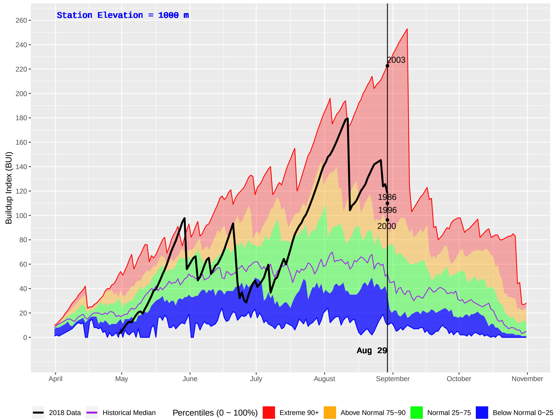
SUCCOUR CREEK (374) : Historical (1986–2016) and Current (2018) Daily Buildup Index (BUI)
